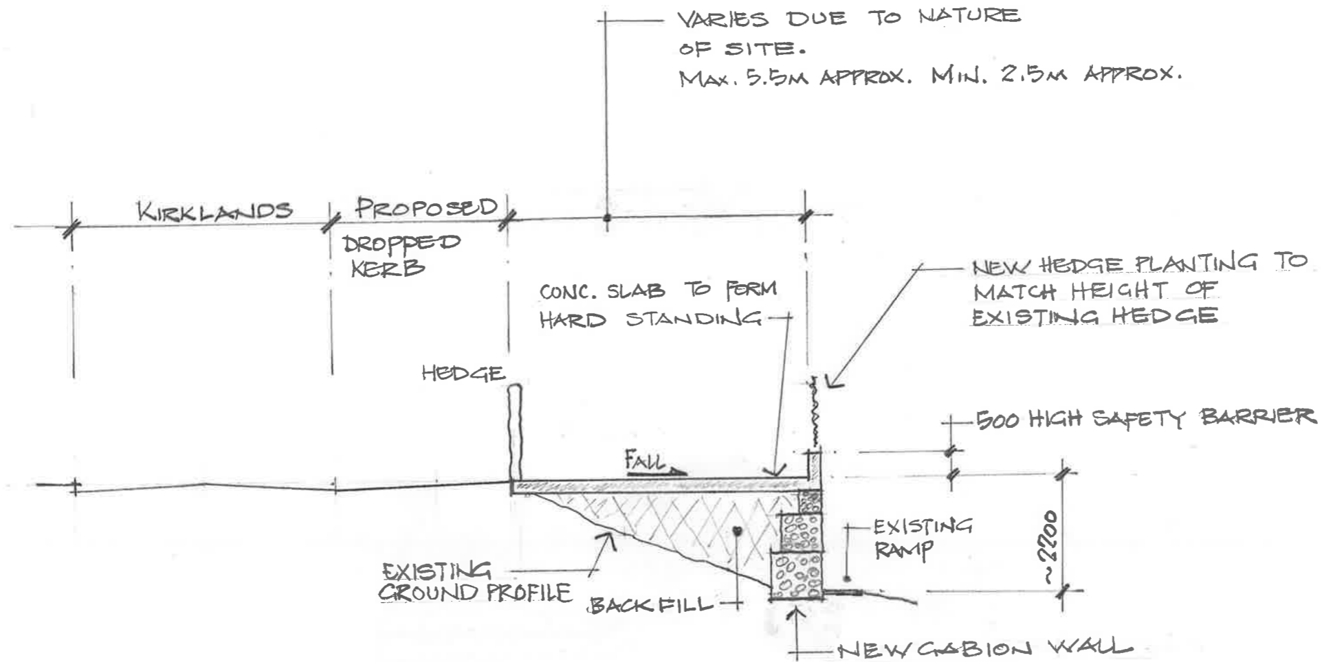
SECTION THROUGH PROPOSED DROPPED KERB/HARD STANDING SCALE 1:100 AT A3
